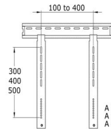
A1= 400 mm x 300 mm Also showing the various size of vertical arms 300 mm, 400 mm & 500 mm
