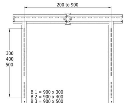
A 1 = 400 x 300 A 2 = 400 x 400 A 3 = 400 x 500
